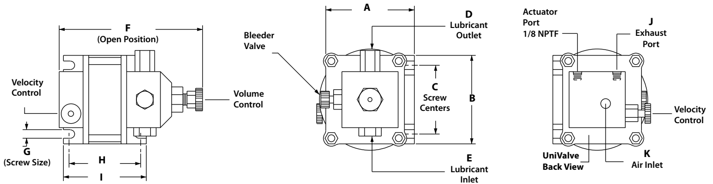
PresSpray Ejector Dimensions.
