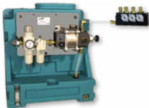
P735-BC w/Remote Manifold Manifold supplied with 6 feet of tubing and fittings.
