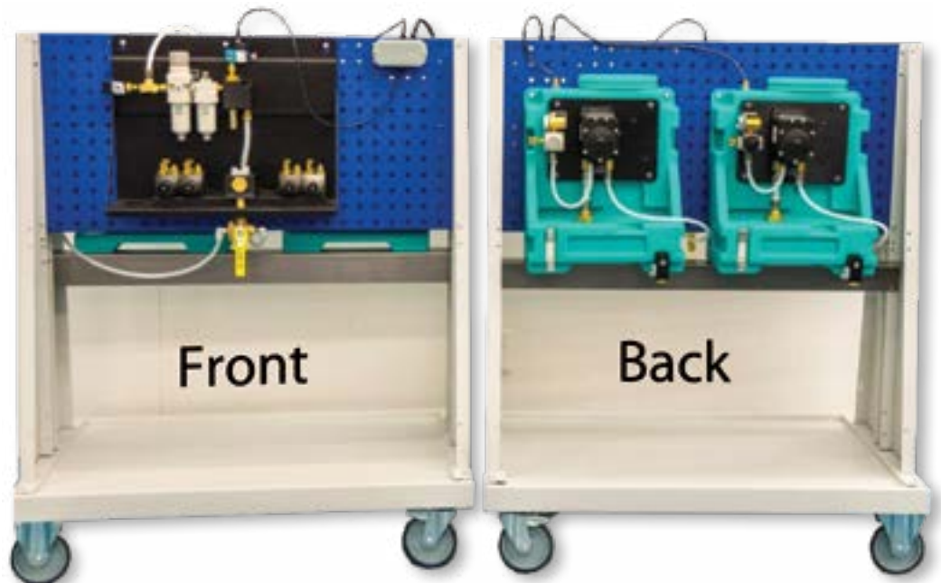
One PresSpray system with two reservoirs mounted on a cart. The PresSpray is shown in the left picture, which is the front of the cart. Two reservoirs are shown mounted on the backside of the cart. This allows user to switch between different lubricants by just turning a valve under the PresSpray to go from one lubricant to another.
