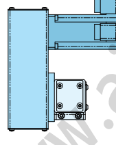
REDUCTION DRIVE TOP RIGHT (SDTR) mounting surface for load shown UP
